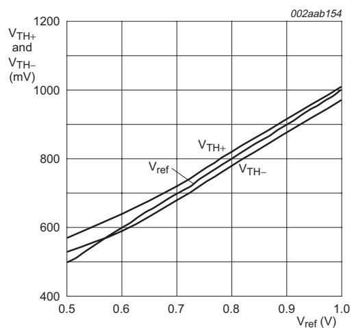
Fig 4. GTL V_{TH+} and V_{TH-} versus V_{ref} ; T_{amb} = -40\text{ }^{\circ}\text{C}
