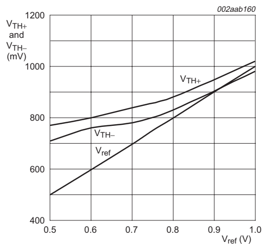
Fig 6. GTL V_{TH+} and V_{TH-} versus V_{ref} ; T_{amb} = +85 °C
